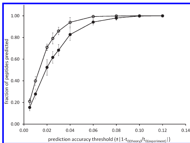
Figure 3. Plots showing the fraction of database peptides predicted accurately for given prediction threshold values. Open- and solid-circles represent data obtained from predictions with intrinsic size parameters and predictions obtained from a polynomial fit to t_D versus molecular weight data, respectively. Data points represent average values obtained from peptide sequences ranging in length from 7 to 15 amino acid residues. Error bars represent one standard deviation from the mean. Prediction accuracy threshold ( x -axis) represents the deviation from the experimental values expressed as a fraction; a prediction accuracy threshold of x = 0.03 would provide the fraction of all database peptides predicted to within \pm 3\% of the experimental values.
