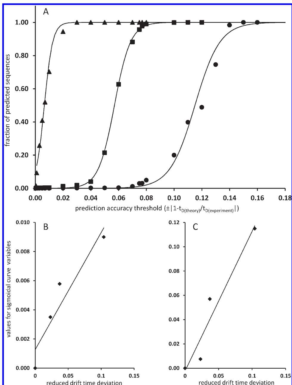
Figure 4. (A) Fraction of all possible 7-,8-,9-, and 10-residue sequences meeting or exceeding the prediction thresholds (x-axis) for t_D s of the select peptide ions [EAYVPATK + 2H] 2+ (solid circles), [QAYAVSEK + 2H] 2+ (solid squares), [LNLFLSTK + 2H] 2+ (solid triangles). Because these values show the overlap between all possible sequences of the same m/z and the correct prediction, the value can be thought of as a false discovery rate (see text for details). Unique peptide ions from the complete list of all possible peptide ions that are within 0.01 Da of the select peptides are used in this analysis. The three different data sets have been fitted with sigmoidal curves (solid traces) using eq 6. (B) w values (eq 6) for the three different curves as a function of reduced t_D deviation, d (see text for details) as well as a zero value. Also shown is a linear least-squares fit of the data (solid line). Plot C shows the x_0 values (eq 6) for the three different curves as a function of d (see text for details) as well as a zero value. Also shown is a linear least-squares fit of the data (solid line).
