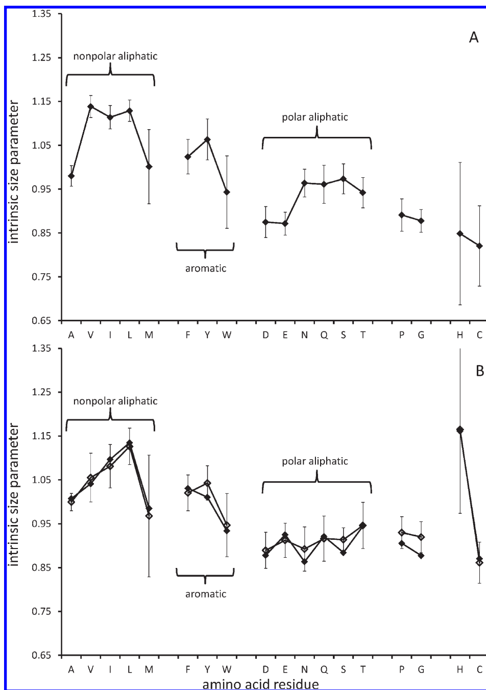
Figure 1. (A) Intrinsic amino acid size parameters derived from a group of doubly charged peptide ions that are 12 residues in length and each contain a single, c-terminal arginine residue. Intrinsic size parameters have been grouped by types of amino acids. Size parameters for proline and glycine are presented separately in light of their propensity to disrupt \alpha -helical structure in solution. Histidine and cysteine size parameters are also shown separately because of their relative infrequent occurrence in the proteome database. Error bars represent one standard deviation about the mean. (B) Average size parameters obtained from doubly charged peptide ions of different residue lengths. Solid and open diamonds represent average values for lysine- and arginine-terminated peptide ions, respectively. Error bars represent one standard deviation from the mean.
